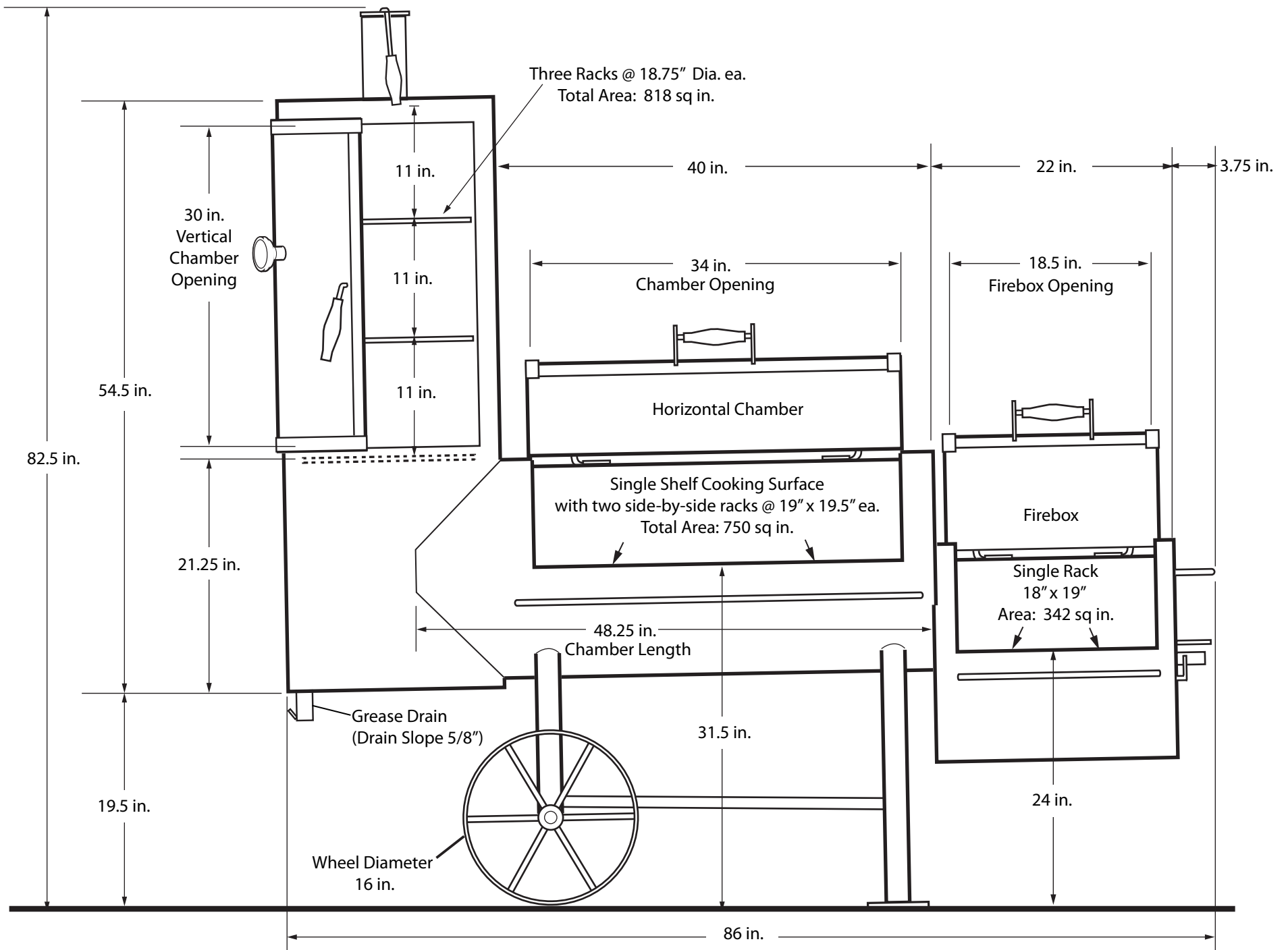
Durango 20" Single Shelf Smoker - Front View
